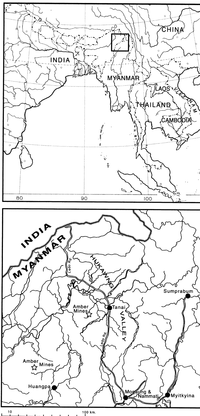
Fig. 1. Location of Burmese amber deposits. Above: inset shows approximate area in southeast Asia. Below: detail within inset.
